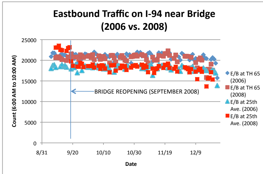
Figure 4.13: Eastbound traffic along I-94 near I-35W (2006 versus 2008)
