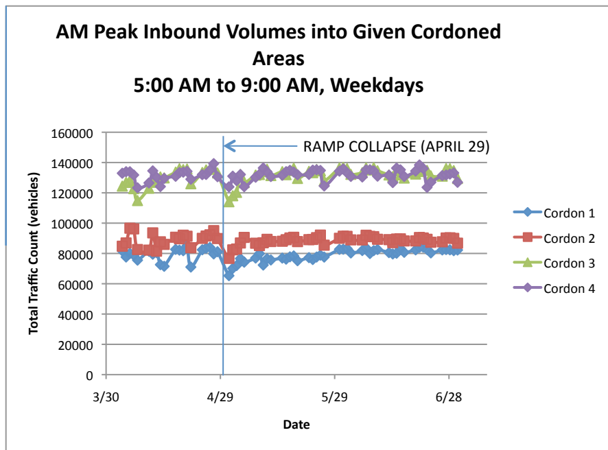
Figure 4.6: Total traffic counts for each cordon circle for Bay Area network
