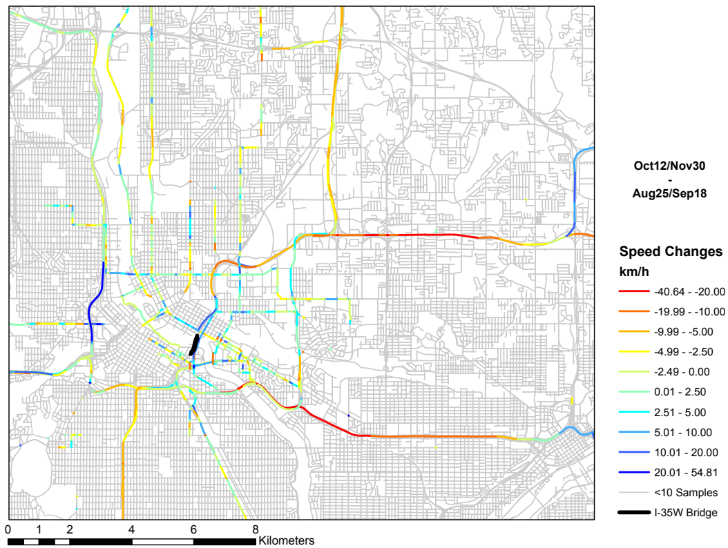
Speed Changes during Morning Peak Period after the Fourth Lane on I-94 Bridge Removed
